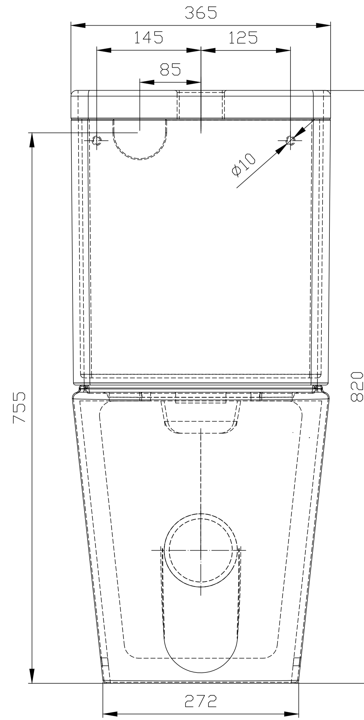
FRONT VIEW
